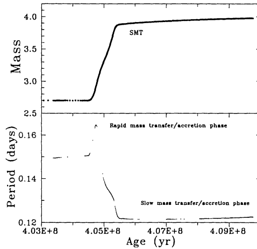
Figure 2. The evolutionary accretion-driven mass changes of a mass-accreting component (upper panel) and calculated pulsation period changes for fundamental radial oscillations (lower panel) in the 2.7M_{\odot} mass-accreting component of a 3M_{\odot} + 2.7M_{\odot} binary system. Evolutionary calculations of binary systems (De Greeve, 1993) were used.
