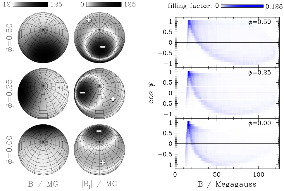
Figure 2. Distribution of the total magnetic field strength B and its longitudinal component B_l on the white dwarf in HE 1045-0908 at (arbitrary) rotational phases \Phi = 0.0, 0.25 , and 0.5 ( left ) and frequency distribution of B and the viewing direction cosine \cos \Phi ( right ).
