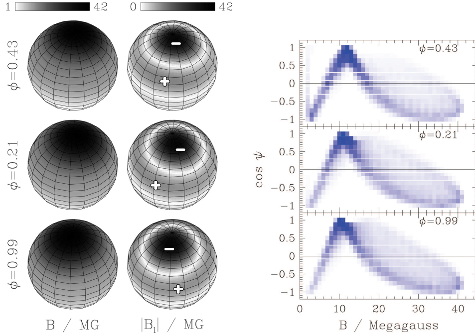
Figure 6. Distribution of the total magnetic field strength B and its longitudinal component B_l on the white dwarf in CP Tuc at rotational phases \Phi = 0.99 , 0.21 , and 0.43 (left) and frequency distribution of B and the viewing direction cosine \cos \Phi (right).
