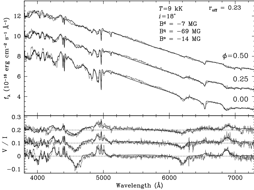
Figure 1. Flux ( top ) and circular polarization ( bottom ) spectra of HE 1045-0908 at (the arbitrary) rotational phases \Phi = 0.0 , 0.25 , and 0.5 . The synthetic spectra for the best-fit model ( thick line ) consisting of a dipole, quadrupole, and octopole field component is shown superimposed on the observed spectra ( grey curve ). For clarity, the upper two flux spectra have been offset by 2 and 4 flux units, respectively, and the polarization spectra by 0.1 and 0.2 units, respectively.
