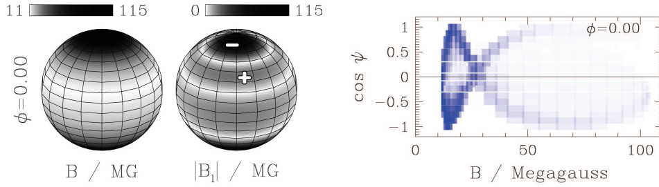
Figure 4. Distribution of the total magnetic field strength B and its longitudinal component B_1 on the white dwarf in EF Eri at spin phase \Phi = 0.0 ( left ) and frequency distribution of B and the viewing direction cosine \cos \Phi ( right ).
