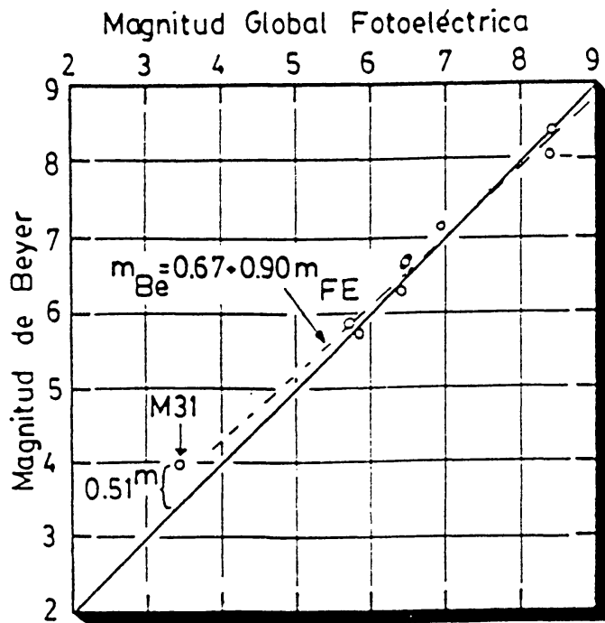
Figure 6. Comparison of Beyer's measurements of extended objects vs their real photoelectric magnitude. The line at 45 degrees would indicate perfect agreement. The mean error of these measurements is only 0.17 magnitudes. M31 departs from the line due to the "Delta Effect" (see text).
